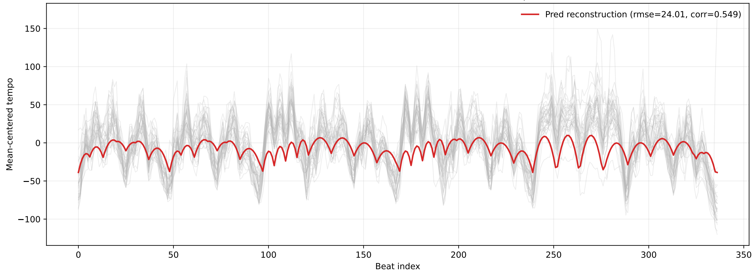
M06-1: Pred reconstruction vs ALL mean-centered true tempo curves
