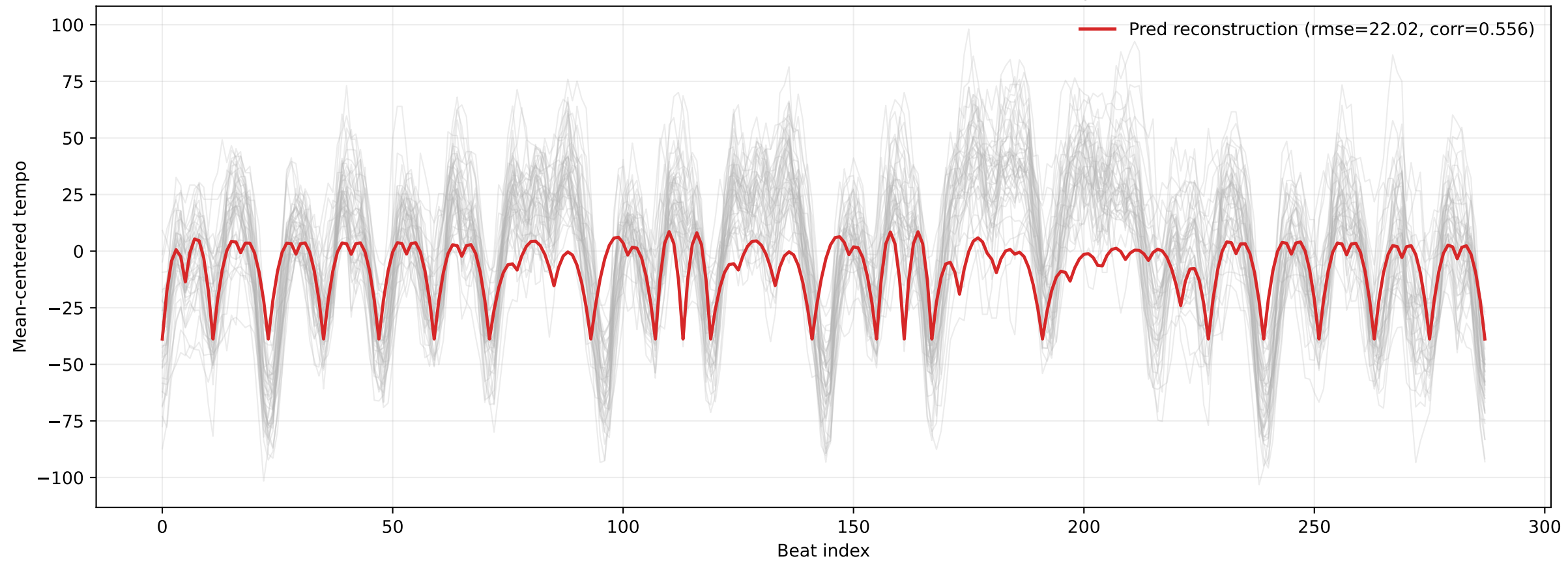
M06-2: Pred reconstruction vs ALL mean-centered true tempo curves
